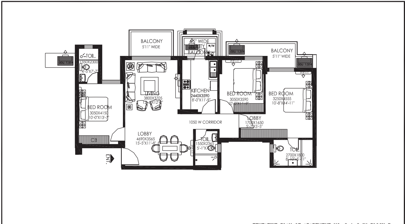
TENTATIVE PLAN OF APARTMENT NO. 2 & 3 IN BLOCK B
