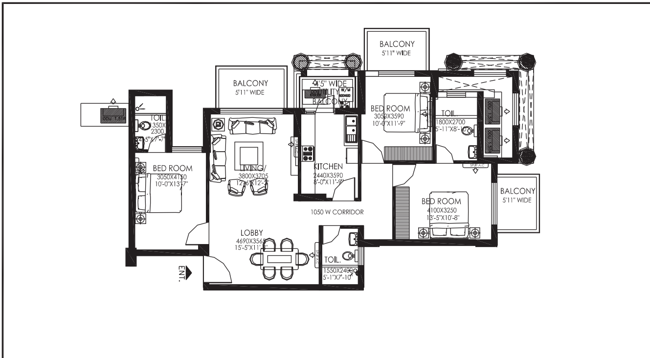
TENTATIVE PLAN OF APARTMENT NO. 3 IN BLOCK A
