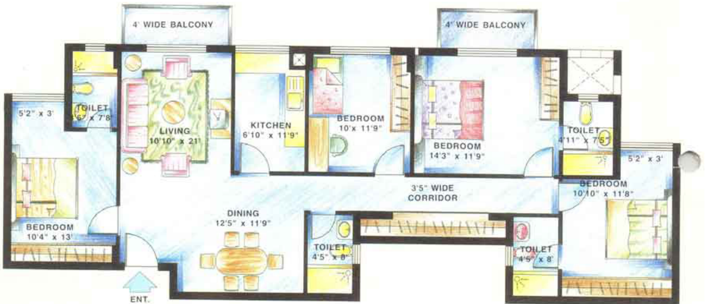
UNIT 1: ACCOMMODATION: Living-Dining, 4 Bedrooms, Kitchen, 4 Toilets and 2 Balconies. AREA: 1682 sq.ft.
