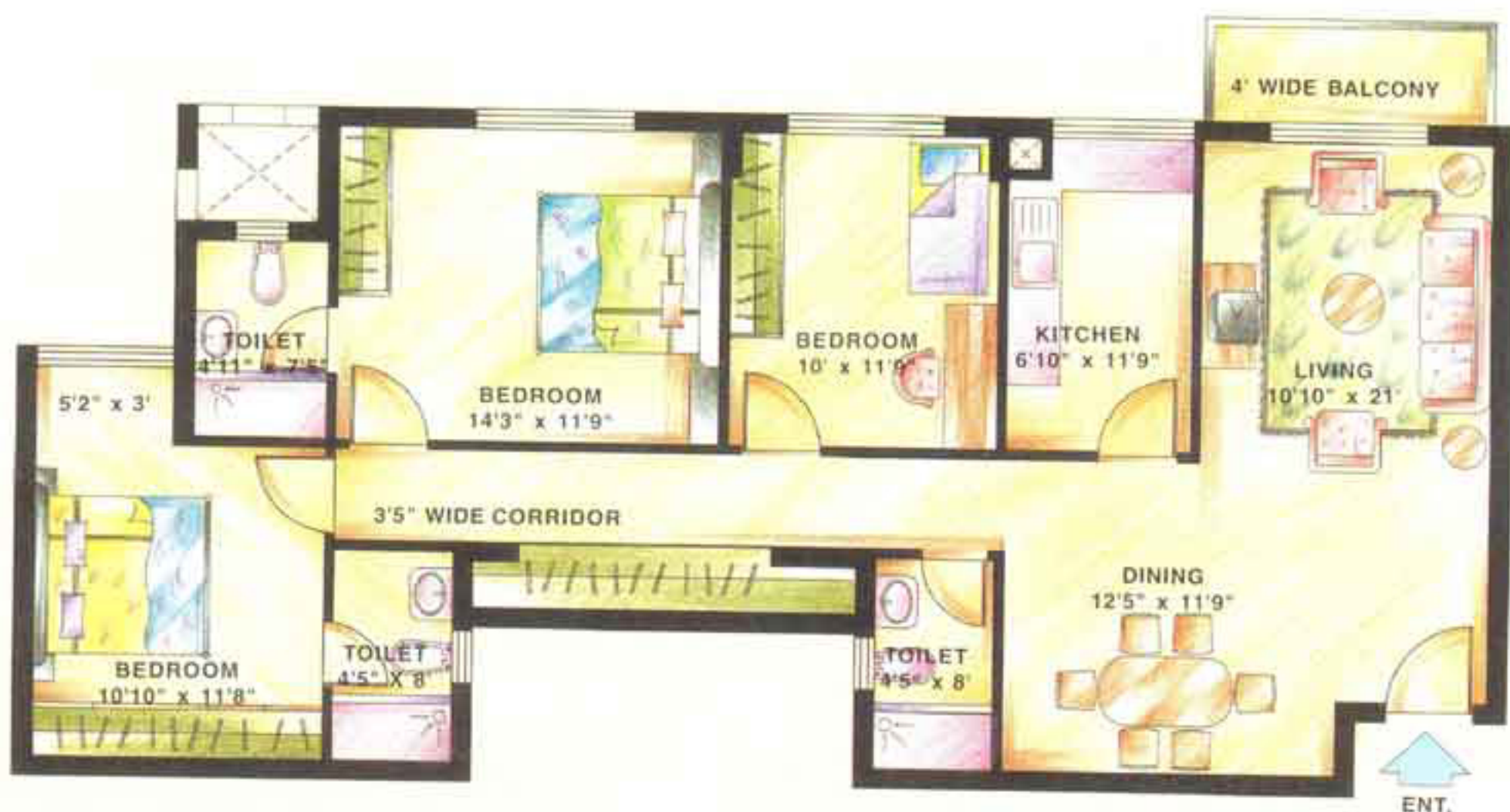
UNIT 2: ACCOMMODATION: Living-Dining with Balcony, 3 Bedrooms, Kitchen and 3 Toilets. AREA: 1396 sq.ft
