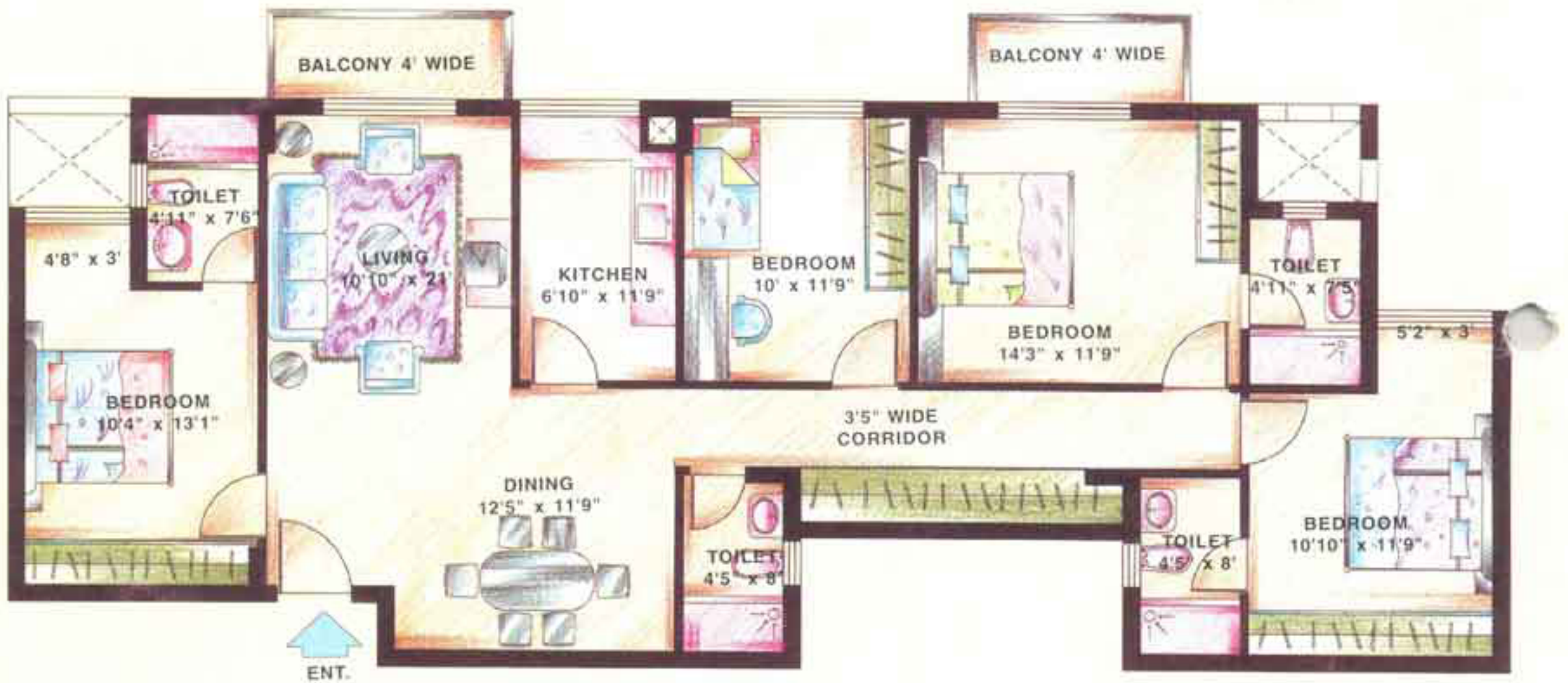
UNIT 5: ACCOMMODATION: Living-Dining, 4 Bedrooms, Kitchen, 4 Toilets, 2 Balconies. AREA: 1682 sq.ft.
