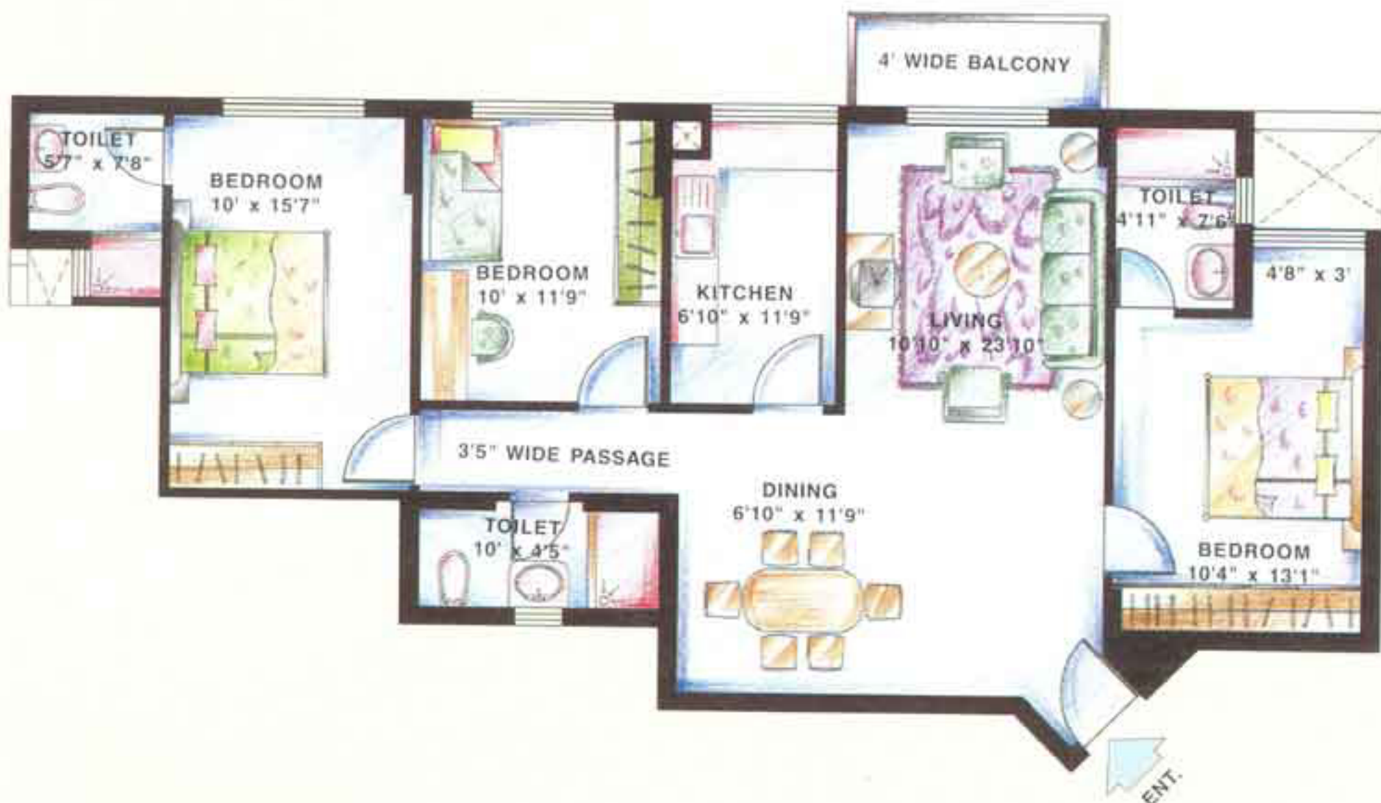
UNIT 4: ACCOMMODATION: Living-Dining with Balcony, 3 Bedrooms, Kitchen and 3 Toilets. AREA: 1346 sq.ft.
