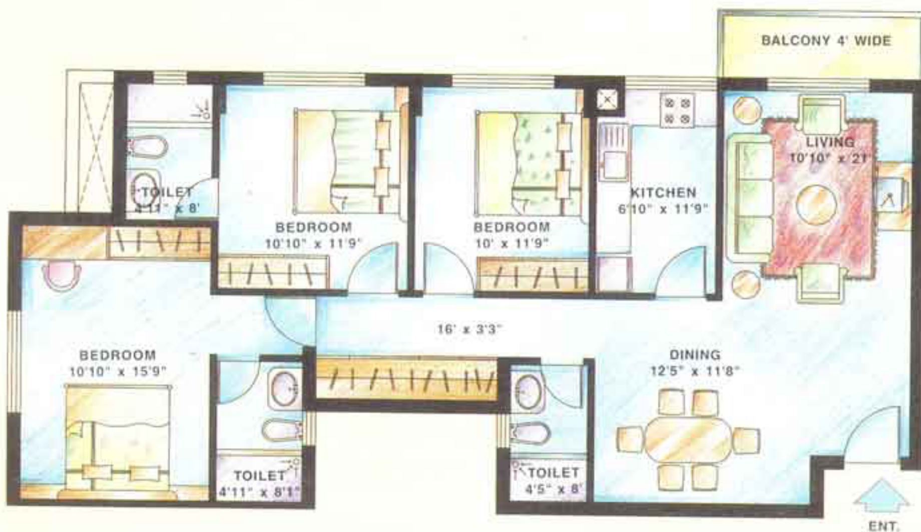
UNIT 2: ACCOMMODATION: Living-Dining with Balcony, 3 Bedrooms, Kitchen and 3 Toilets. AREA: 1376 sq.ft.
